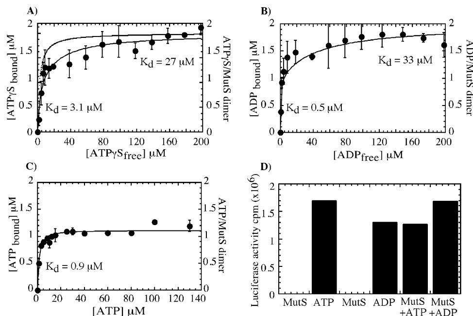
FIGURE 1: T. aquaticus MutS dimer binds two nucleotides with differing affinities. In panel A, ^{35}\text{S} -ATP \gamma S binding to MutS (1 \mu\text{M} dimer) was measured by nitrocellulose membrane filtration. One ATP \gamma S molecule binds MutS with high affinity ( K_d = 3 \pm 0.6 \mu\text{M} ), and a second one binds with lower affinity ( K_d = 27 \pm 8 \mu\text{M} ). In panel B, similarly, two ADP molecules bind MutS with differing affinities ( K_d = 0.5 \pm 0.05 and 33 \pm 5 \mu\text{M} ). In panel C, Only one ATP binding to MutS is detectable ( K_d = 0.9 \pm 0.2 \mu\text{M} ). In panel D, bioluminescence assays performed with heat-denatured MutS indicate no tightly bound ATP or ADP contaminants in the preparation, as 100 nM MutS alone yields luciferase activity equivalent to 39 \text{ cpm} compared with 1.69 \times 10^6 \text{ cpm} for 100 nM ATP and ADP standards, respectively. In control experiments, exogenous addition of 100 nM ATP or ADP to MutS yields luciferase activity equivalent to 1.35 \times 10^6 and 1.68 \times 10^6 \text{ cpm} , respectively.
