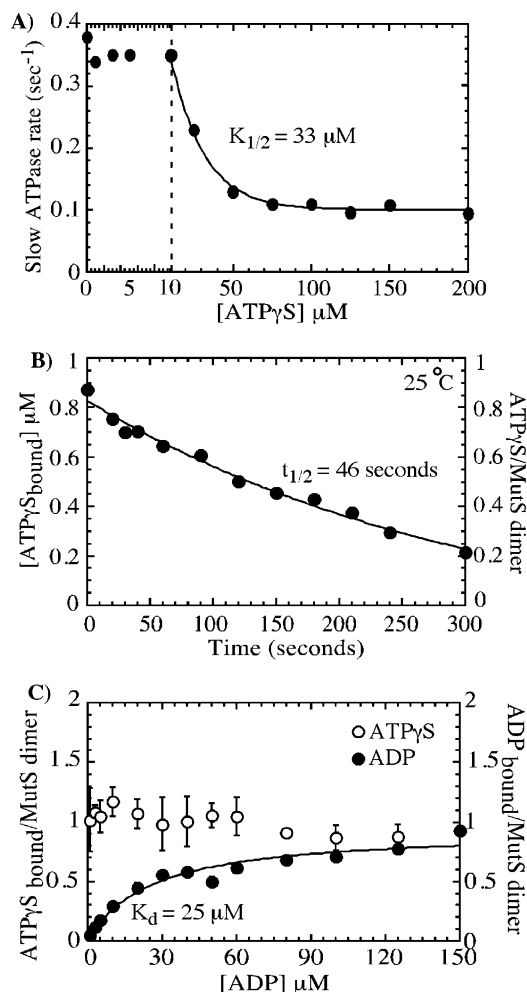
FIGURE 4: The low-affinity site on ATPγS-bound MutS hydrolyzes ATP slowly, yielding an ATPγS–ADP-bound MutS dimer species. In panel A, further analysis of the data in Figure 3 shows that inhibition of the slow ATPase phase (rate constant = 0.3\text{--}0.4 \text{ s}^{-1} ) requires higher ATPγS concentrations, and the plot of rate constants versus ATPγS fit to a hyperbola yields K_{1/2} = 33 \mu\text{M} (similar to the K_d of 27 \mu\text{M} for ATPγS binding to the low-affinity site on MutS, see Figure 1A); ATPase data for 150 \mu\text{M} ATPγS are shown in Figure 3D. In panel B, a nitrocellulose filter-binding experiment, in which ^{35}\text{S} -ATPγS ( 12 \mu\text{M} ) bound to MutS ( 1 \mu\text{M} dimer) is chased by ATP ( 500 \mu\text{M} ), shows that ATPγS dissociates from MutS at a very slow rate of 0.015 \text{ s}^{-1} ( t_{1/2} = 46 \text{ s} ); that is, it remains bound to the MutS high-affinity site during the slow ATPase phase. In panel C, MutS ( 1 \mu\text{M} dimer) preincubated with ^{35}\text{S} -ATPγS (○; 5 \mu\text{M} ) and titrated with ^{32}\text{P} -ADP (●; 0\text{--}150 \mu\text{M} ) shows binding of one ADP molecule to the low-affinity site ( B_{\text{max}} = 0.93 \pm 0.06 \mu\text{M} and K_d = 25 \pm 5 \mu\text{M} ) and retention of the ATPγS molecule already bound to the high-affinity site.
