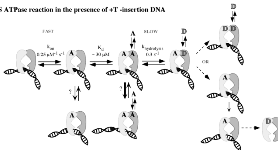
FIGURE 7: Prominent species in the MutS ATPase pathway and their interactions with DNA. According to the kinetic parameters measured for MutS ATPase, in the absence of DNA or in the presence of fully matched DNA, the first slow, rate-limiting step occurs after ATP hydrolysis at S1, indicating that S1_{ADP}-S2_{ATP} might be a stable species in this pathway. In contrast, when MutS is bound to a DNA mismatch, the first rate-limiting step occurs prior to ATP hydrolysis at S1, indicating that S1_{ATP}-S2_{ATP} and perhaps S1_{ATP}-S2_{ADP} as well might be the stable species in this ATPase pathway. The model also depicts possible interactions between various nucleotide-bound MutS species and mismatched DNA based on results from DNA-binding experiments in this study and in the literature. Dashed arrows indicate steps that may not happen in immediate succession.
