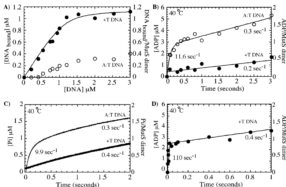
FIGURE 5: Mismatched DNA suppresses ATP hydrolysis. In panel A, nitrocellulose membrane filtration experiments with 1 \mu\text{M} MutS dimer titrated with ^{32}\text{P} -DNA show near 1:1 stoichiometric interaction between MutS and DNA containing a +T insertion but significantly weaker interaction with fully matched DNA. In panel B, preincubation of MutS (3 \mu\text{M} dimer) with mismatched DNA (5 \mu\text{M} ) results in complete inhibition of the burst of ATP hydrolysis (●); ATP hydrolysis in the presence of fully matched DNA (○; burst rate constant = 11.6 \pm 2 \text{ s}^{-1} and amplitude = 2.7 \pm 0.1 \mu\text{M} or one ADP per MutS dimer) is the same as in the absence of DNA (see Figure 2C). In panel C, phosphate-release kinetics of MutS (1 \mu\text{M} dimer) confirm that ATP hydrolysis is suppressed by +T DNA and not by fully matched DNA and that the phosphate-release rates remain fast even in the presence of DNA. In panel D, pulse-chase analysis reveals rapid ATP binding to the MutS+T DNA complex at 0.22 \mu\text{M}^{-1} \text{ s}^{-1} followed by slow hydrolysis, confirming that mismatched DNA specifically inhibits the ATP hydrolysis step.
