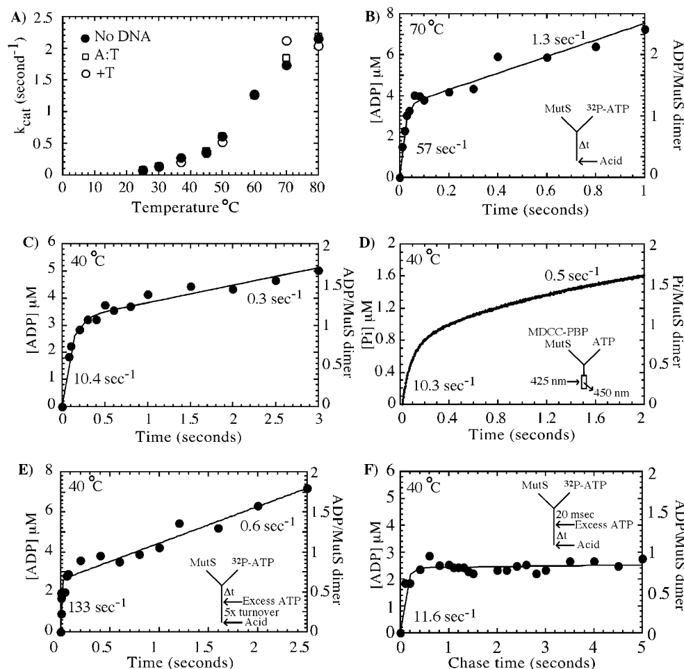
FIGURE 2: Asymmetry in ATP binding is recapitulated during ATP hydrolysis. In panel A, steady-state ATPase activity of T. aquaticus MutS is temperature-dependent with k_{cat} approaching a maximum of 2 s -1 at 80 °C. In panel B, pre-steady-state rapid-quench analysis of MutS activity at 70 °C reveals a burst of ATP hydrolysis at a rate of 57 \pm 11 s -1 and amplitude of 3.5 \pm 0.15 μM, followed by a slow steady-state phase at 1.3 \pm 0.12 s -1 (3 μM MutS dimer and 500 μM ATP in the reaction). The burst phase is equivalent to rapid hydrolysis of one ATP molecule per MutS dimer. In panel C, the burst rate and k_{cat} vary with temperature (e.g., at 40 °C the burst rate constant is 10.4 s -1 and the linear rate constant is 0.3 s -1 , although the amplitude is still 3.2 μM, see Table 1). In panel D, a fluorescent reporter assay measures a burst of phosphate release from 1 μM MutS at 10.3 \pm 0.3 s -1 at 40 °C and 1.1 ± 0.02 μM amplitude (one ADP/P i per MutS dimer), suggesting that the phosphate is released rapidly following ATP hydrolysis. In panel E, pulse-chase experiments at 40 °C with 3 μM MutS and 500 μM ATP also show a burst amplitude of one ADP per dimer and yield an ATP binding rate constant of 0.25 \pm 0.1 μM -1 s -1 . In panel F, a pulse-chase time experiment, in which hydrolysis of 32 P-ATP (500 μM) bound to MutS (3 μM dimer) prior to addition of unlabeled ATP chase (10 mM) is observed over time, detects only one ADP formed per MutS dimer in the first turnover (burst rate = 11.6 \pm 2.3 s -1 ).
