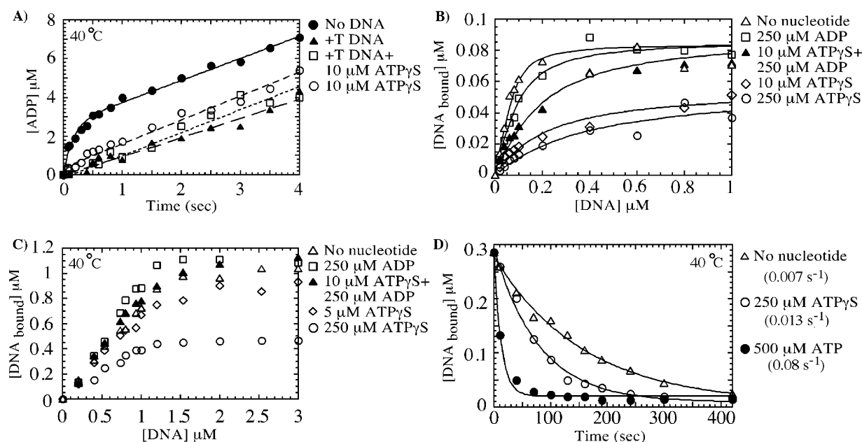
FIGURE 6: Mismatched DNA inhibits ATP hydrolysis specifically at the high-affinity site, yielding an ATP/ADP-bound form of MutS, which has high affinity for mismatched DNA. In panel A, +T DNA binding to MutS (3 \mu\text{M} dimer) suppresses the burst of ATP hydrolysis (▲), but the slow phase remains identical to that in the absence of DNA (●, 0.33 \text{ s}^{-1} ). The same slow ATPase rate is observed for MutS preincubated with 10 \mu\text{M} ATP \gamma S (○, high-affinity site occupied, no burst phase) or with 10 \mu\text{M} ATP \gamma S and +T DNA (□), indicating that the low-affinity site continues to hydrolyze ATP when MutS is bound to mismatched DNA. Panels B and C show nitrocellulose membrane filtration experiments of 0.1 and 1 \mu\text{M} MutS dimer, respectively, binding to +T DNA in the absence of nucleotide cofactors (Δ, K_d = 20 \text{ nM} ), in the presence of 250 \mu\text{M} ADP (□, both high-affinity and low-affinity sites occupied, K_d = 45 \text{ nM} ), and in the presence of 10 \mu\text{M} ATP \gamma S and 250 \mu\text{M} ADP (▲, ATP \gamma S in high-affinity site and ADP in low-affinity site, K_d = 100 \text{ nM} ). The interaction between MutS and +T DNA is weaker in the presence of 10 \mu\text{M} ATP \gamma S (◇, one site occupied by ATP \gamma S, K_d \approx 200 \text{ nM} ; note stable +T DNA interaction with this species at 1 \mu\text{M} MutS) and 250 \mu\text{M} ATP \gamma S (○, both sites occupied with ATP \gamma S, K_d \approx 300 \text{ nM} ; note weak +T DNA interaction with this species even at 1 \mu\text{M} MutS). In panel D, the rate of dissociation of ^{32}\text{P} -labeled +T DNA (1 \mu\text{M} ) from MutS (0.5 \mu\text{M} ) was measured over time by membrane filtration assays using 50 \mu\text{M} unlabeled +T DNA chase (with or without nucleotides). The dissociation rate is 0.007 \text{ s}^{-1} in the absence of nucleotides (Δ), 0.013 \text{ s}^{-1} in the presence of 250 \mu\text{M} ATP \gamma S (○), and 0.077 \text{ s}^{-1} in the presence of 500 \mu\text{M} ATP (●).
