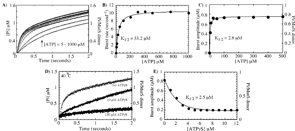
FIGURE 3: The high-affinity ATP-binding site on MutS catalyzes rapid ATP hydrolysis. In panel A, phosphate-release kinetics were measured at increasing ATP concentrations and, in panel B, yielded a maximum burst rate constant of 10.7 \pm 0.2 \text{ s}^{-1} and K_{1/2} = 33.2 \pm 2.5 \mu\text{M} , as well as, in panel C, a maximum amplitude of 0.8 \pm 0.01 \mu\text{M} and K_{1/2} = 2.8 \pm 0.4 \mu\text{M} for 1 \mu\text{M} MutS dimer at 40^\circ\text{C} . In panel D, preincubation of MutS ( 1 \mu\text{M} dimer) with increasing concentrations of ATP \gamma S (0–200 \mu\text{M} ) suppresses the rapid burst of hydrolysis (500 \mu\text{M} ATP in the reaction). In panel E, no burst phase can be detected at ATP \gamma S concentrations higher than 5 \mu\text{M} ; that is, following ATP \gamma S binding to the high-affinity site (see Figure 1A), and a plot of decreasing burst amplitudes versus ATP \gamma S concentration fit to a hyperbola yields K_{1/2} = 2.5 \pm 0.7 \mu\text{M} (similar to the K_d for ATP \gamma S binding to the high-affinity site on MutS, see Figure 1A).
